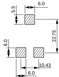
Land Pattern: [mm]
