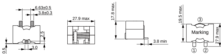
Dimensions: [mm]
