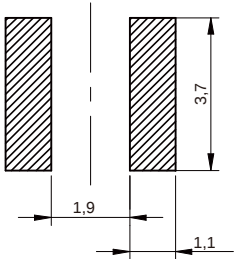
Land Pattern: [mm]
