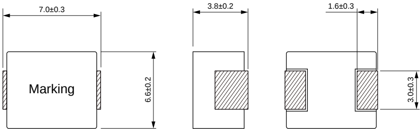
Dimensions: [mm]
