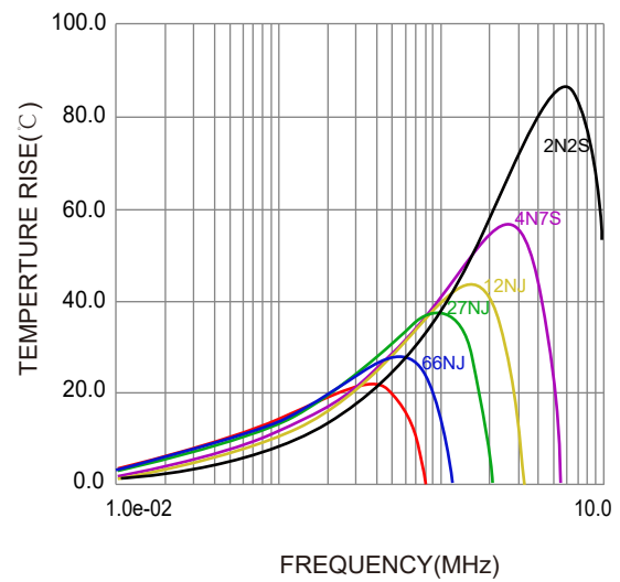
Temperture Rise VS. Frequency Characteristics:
