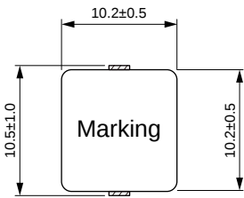
Dimensions: [mm]
