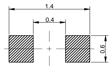
Land Pattern: [mm]
